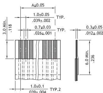
Accommodated FFC
