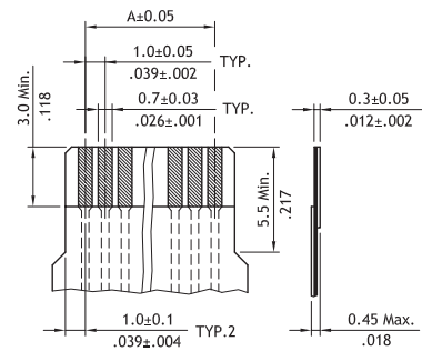
Accommodated FPC
